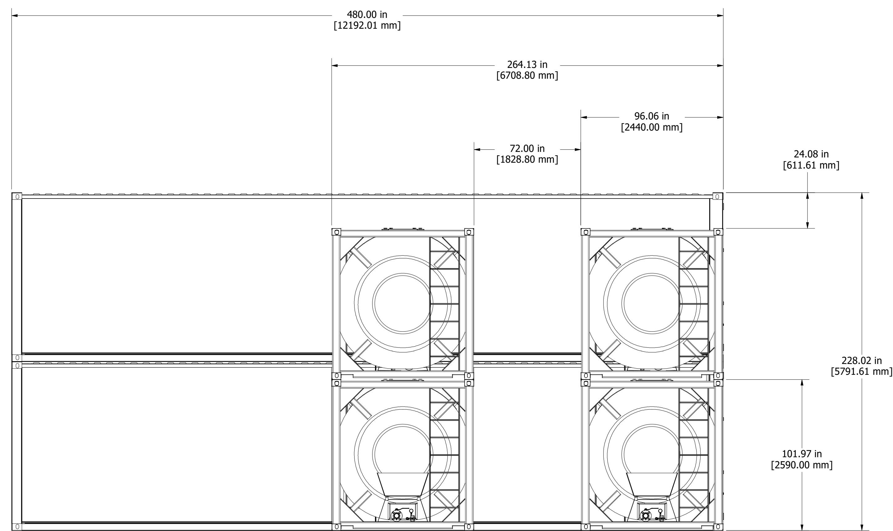
LEFT SIDE VIEW SCALE 1 / 40
