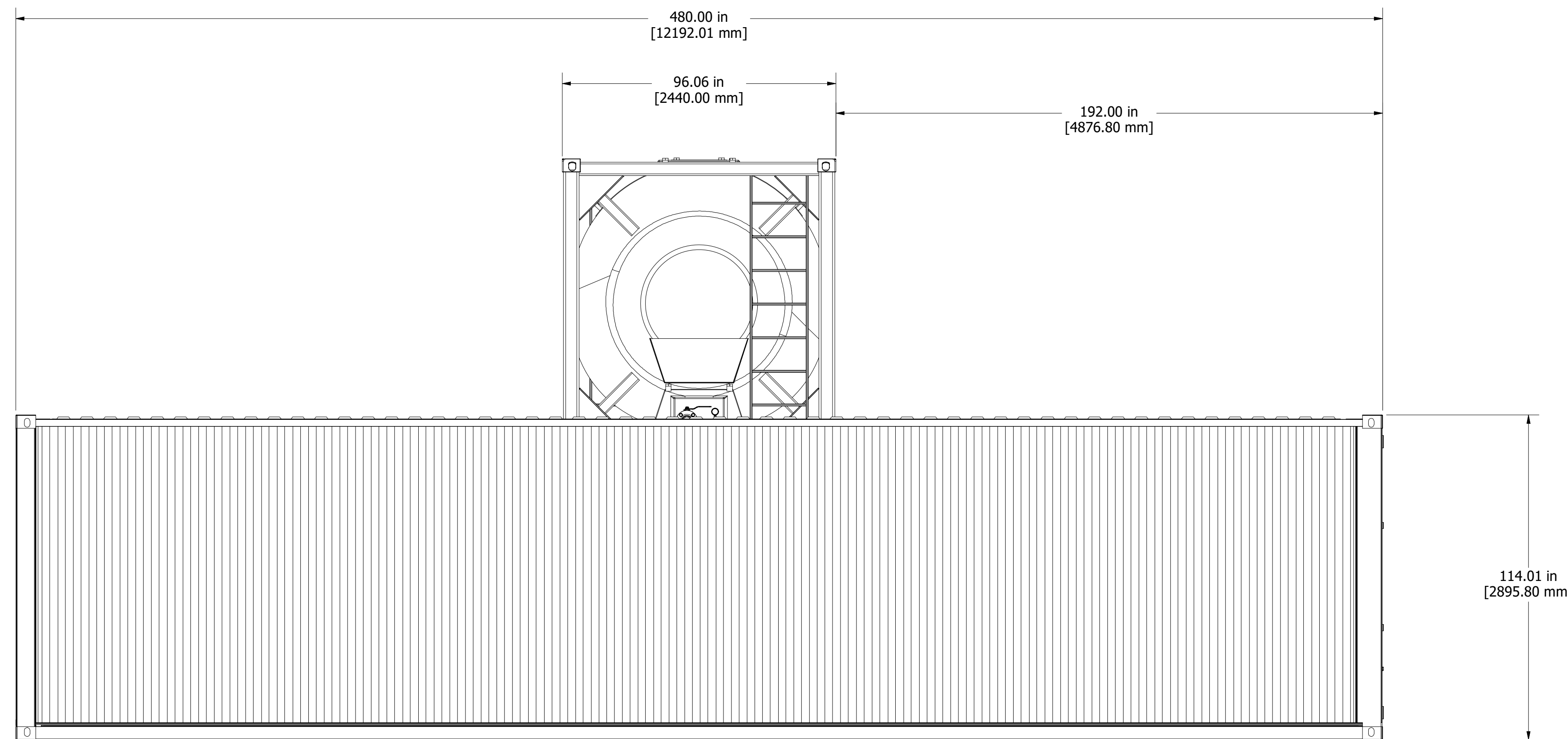
LEFT SIDE VIEW SCALE 1 / 30
