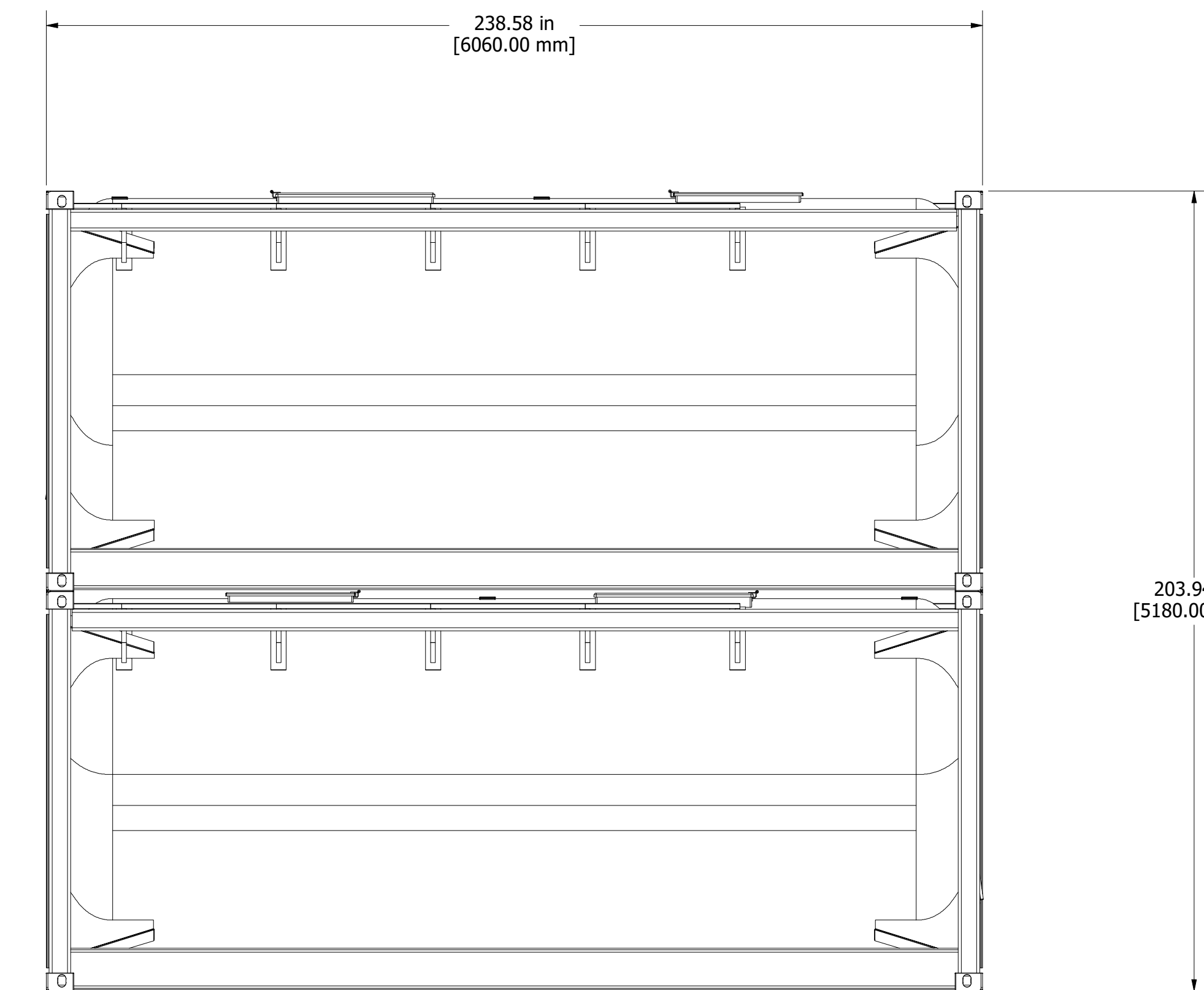
FRONT VIEW SCALE 1 / 30
